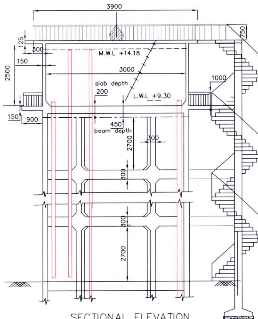
SECTIONAL ELEVATION
